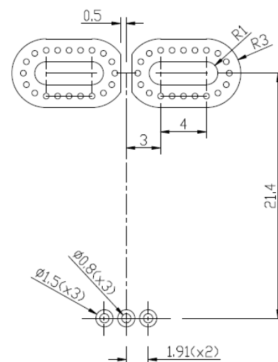
(For reference only) Land Pattern
